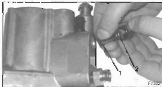
Figure 3 Installing spring and discharge fitting
