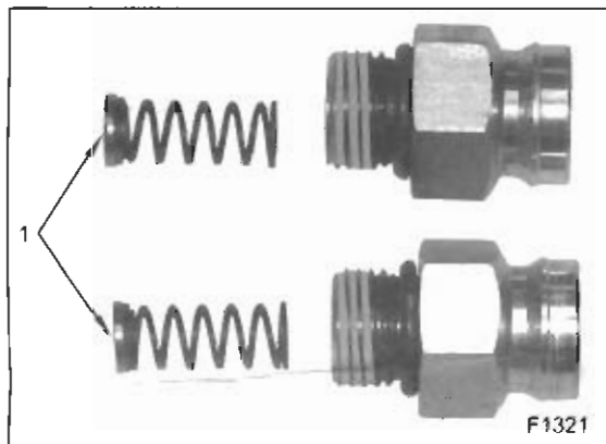
Figure 2 Spring poppet orientation
